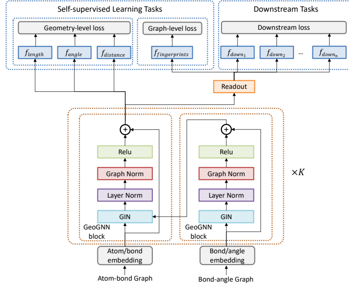
Figure 5: Architecture of GeoGNN.
