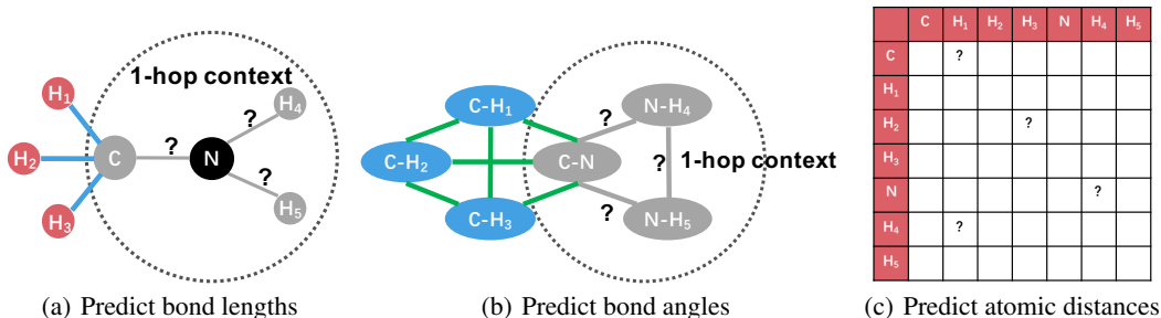
Figure 4: Demonstration of geometry-level self-supervised learning tasks. (The black circle represents the selected atom. The gray circles and lines represent the neighboring masked atoms, bonds, and bond angles.)
