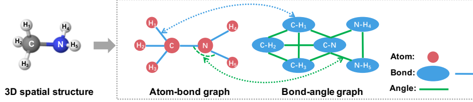
Figure 2: Illustration of the atom-bond graph and the bond-angle graph. The left figure shows the structure of Methanamine in the 3D space. We can easily encode its geometry information with the help of the atom-bond graph that describes the relations between atoms and bonds and the bond-angle graph that describes the relations between bonds and bond angles.
