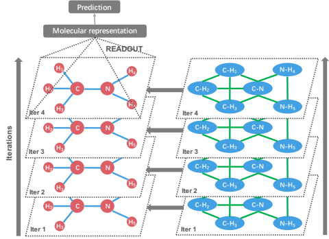
Figure 3: Overall architecture of GeoGNN
