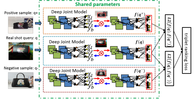
Figure 6: Unified deep ranking framework consists of deep joint models for (q, q^+, q^-) by feeding the triplets into the network.
