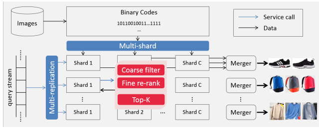
Figure 7: Multi-replications and multi-shards engine architecture for image indexing.
