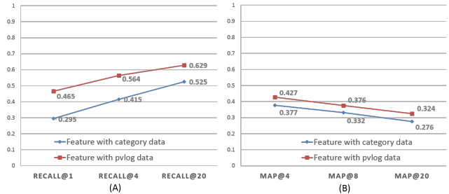
Figure 9: Comparison between feature with category data and pvlog data on A) Recall (B) MAP.
